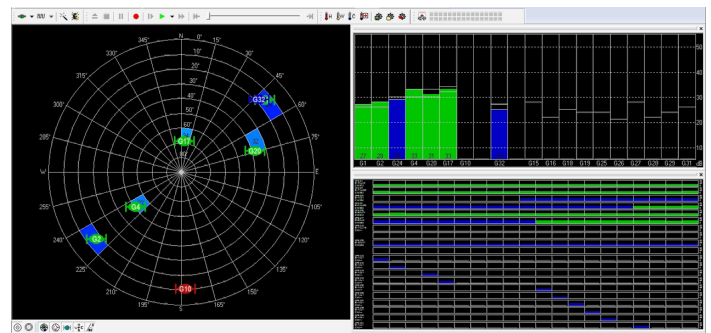
Figure 12 - Screen shot of u-Center while acquiring GPS signal from satellites. Left: sky view of satellite locations, upper right: C/N 0 of each captured satellite, and lower right: satellite levels
