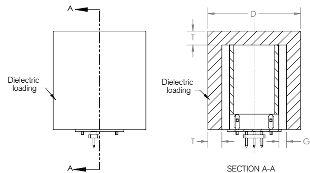
Figure 10 - Cylindrical dielectric loading
