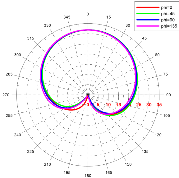
A 117 degree beamwidth ensures excellent hemispherical coverage.
